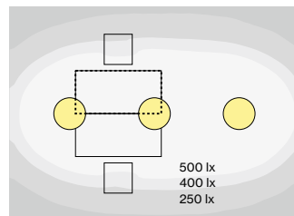
TASK 600 round surface 30W, 4000K, direct
